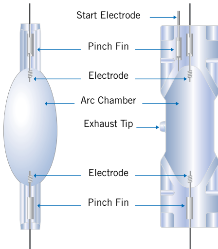
Uni-Form® Formed-body Pulse Start Arc Tube
